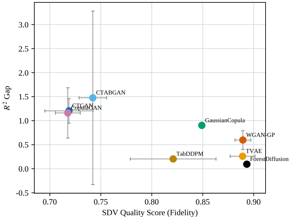
Concrete: SDV Quality Score (Fidelity) vs R^2 Gap
